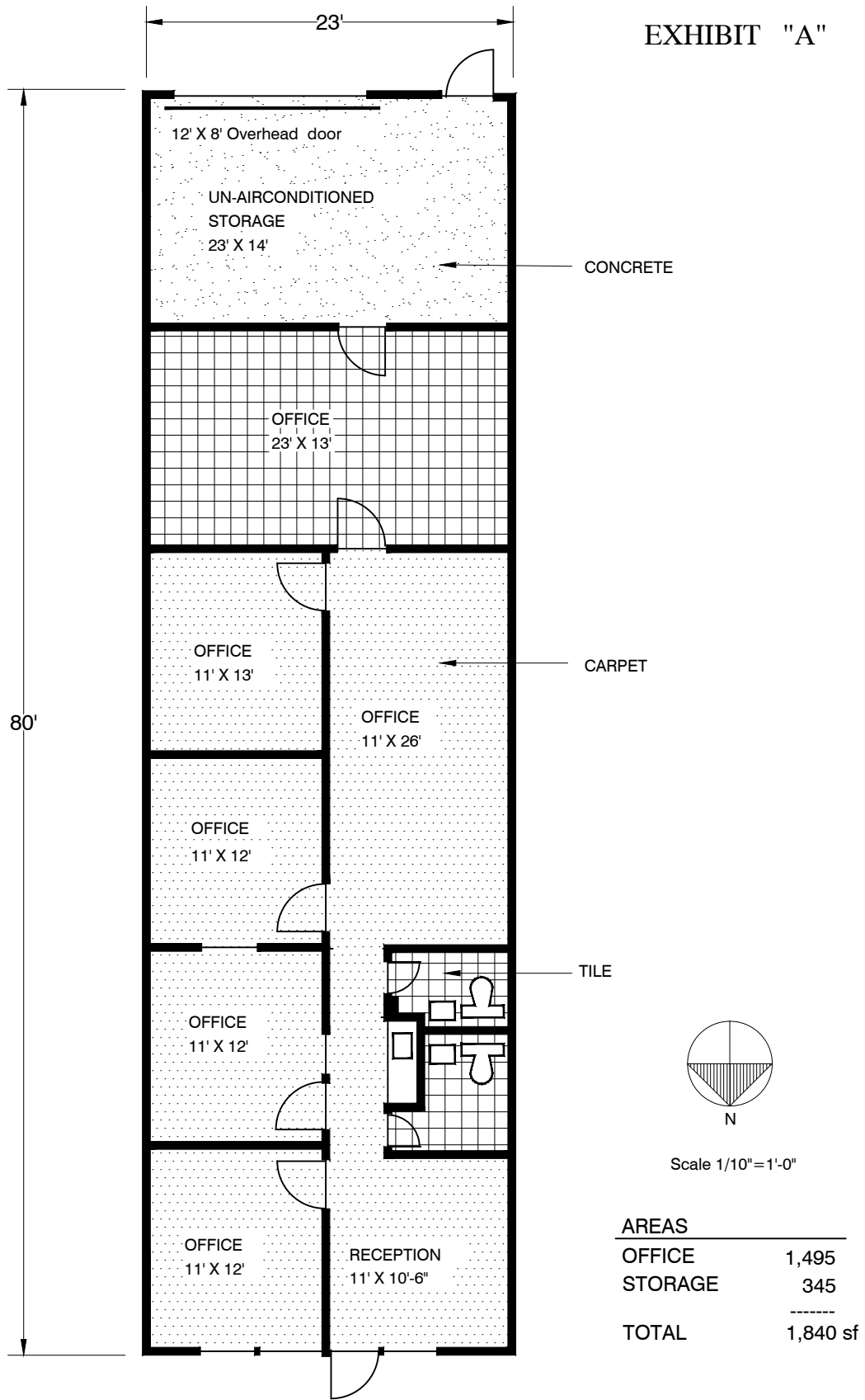
FLOOR PLAN of 1778 WEST SAM HOUSTON PARKWAY NORTH
